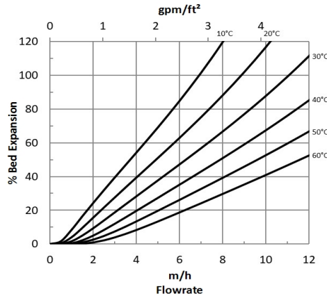
Figure 1b: Backwash Expansion – Anion
